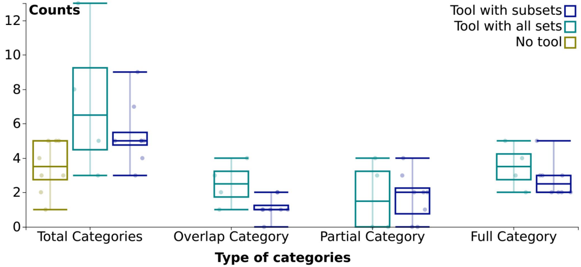
Figure 6: The statistic of categories was generated from 8 participants with an age dataset in (a) and a temperature dataset in (b). The x -axis represents the type of categories such as Overlap Category , Full Category and Partial Category as shown in Fig. 2; Total categories refers to all the generated categories; the y -axis represents the number of each type of categories.
