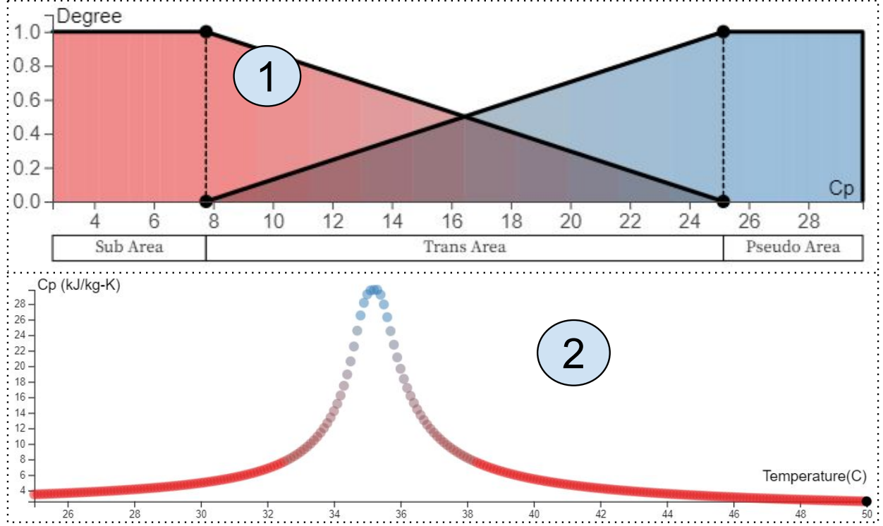
Figure 4: Categorize Specific Heat(Cp) . In ①, the x axis shows Cp and y axis represents the membership degree, which generates two Full Category s. ② shows the relationship between temperature( x axis) and Cp ( y axis) with the scatter plots.
