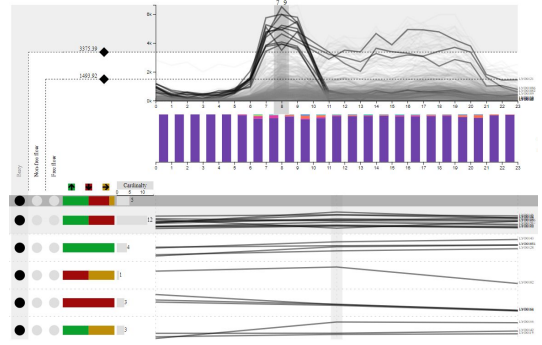
Figure 4: The traffic flow patterns during morning peak. An aggregated group with 5 subgroups reaches the peak time in the morning, but some do not reach the peak in the evening.
