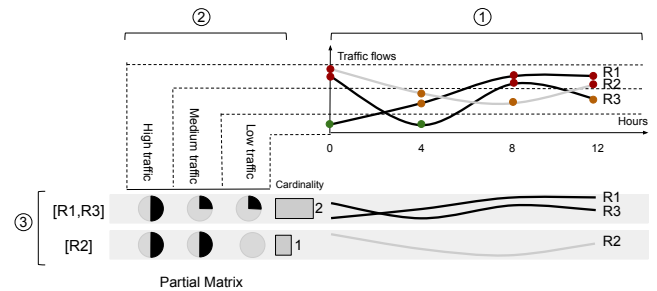
Figure 1: GROUPSET technique overview. Sets are created from time-varying data (line chart) in ①. The same sets are organized as columns to indicate partial membership as pie charts in ② and set intersections are listed as rows to represent groups of similar lines (along with their partial membership representation) in ③.
