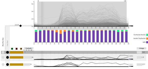
Figure 3: Road segments that are always not busy. An aggregated group with two subgroups contains 64 and 50 road segments that only belong to Free flow during 24 hours.
