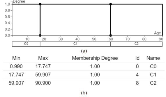
Figure 2: Categorization using crisp membership function, there are three crisp categories generated from the crisp membership function showed in (a) and the detail information of categories in (b).
