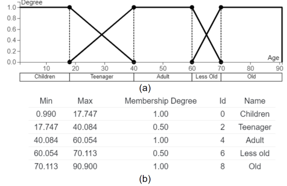
Figure 5: The age data are from 0 to 90, there are three main categories with name Children , Adult and Old . Meanwhile, two fuzzy categories created and they are named with Teenager and Less old .
