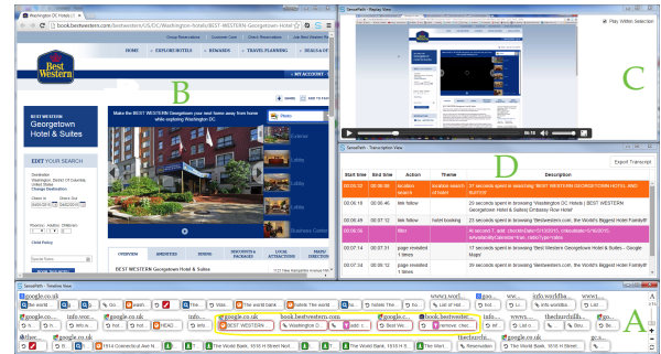
Figure 1: Four linked visualizations of SensePath. A: The timeline view shows all captured sensemaking actions in temporal order. B: The browser view displays the web page where an action was performed. C: The replay view shows the screen capture video to provide additional context. D: The transcription view details selected actions (highlighted in the timeline) and generates their transcript.
