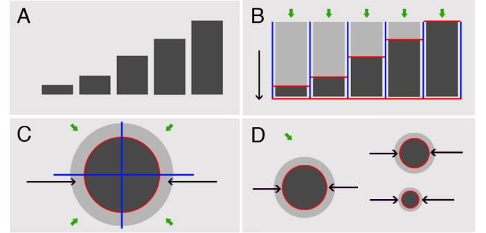
Fig. 5. Template schemas: Blue lines represent the walls ; red lines the ground ; green arrows the entrance point ; black arrow the gravity direction ; light grey shapes the deposit area ; and dark grey shapes the aggregated area . (A) A common bar chart and (B) its template; (C) the pie chart template; (D) the bubble chart template.
